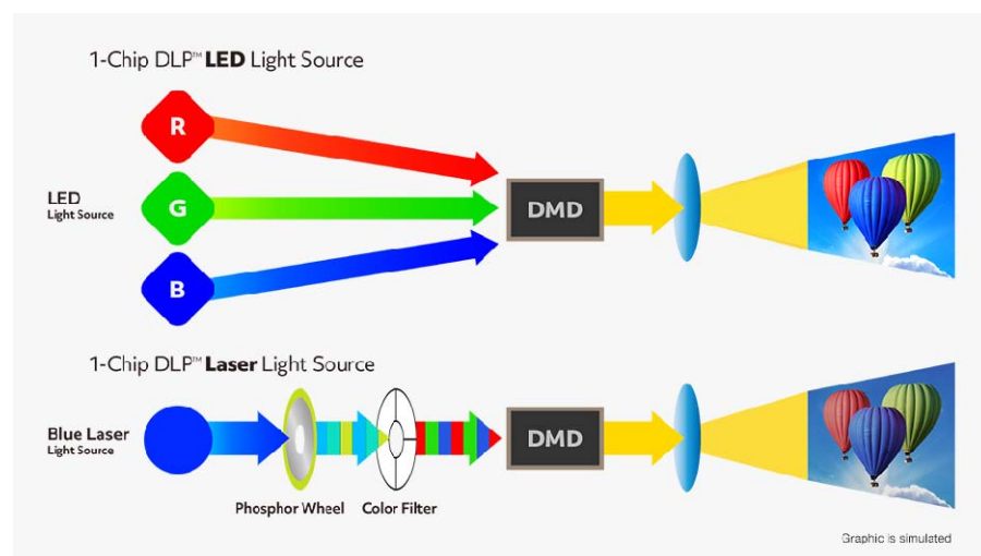
RGB LED Optical Structure Image
